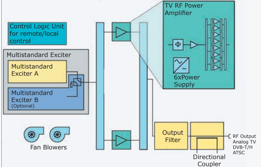
3A5K0A - Functional Block Diagram
