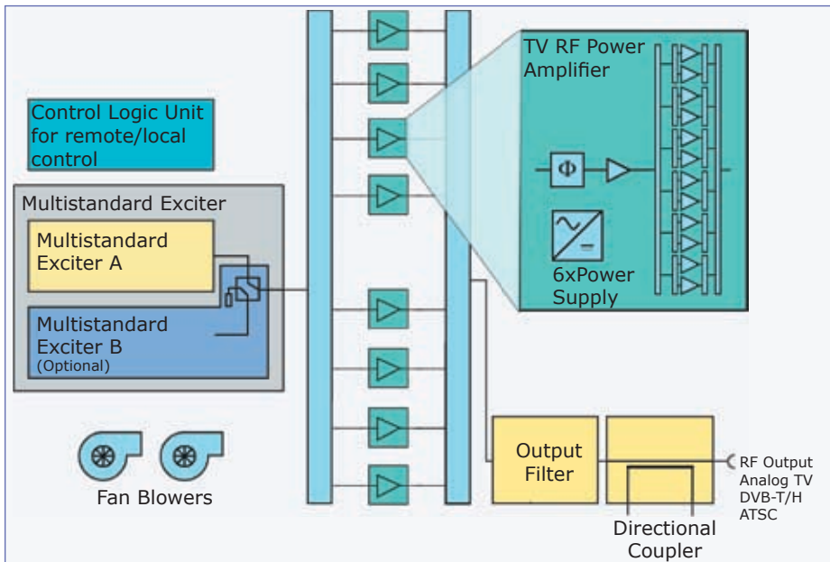
3A20KT Functional Block Diagram
