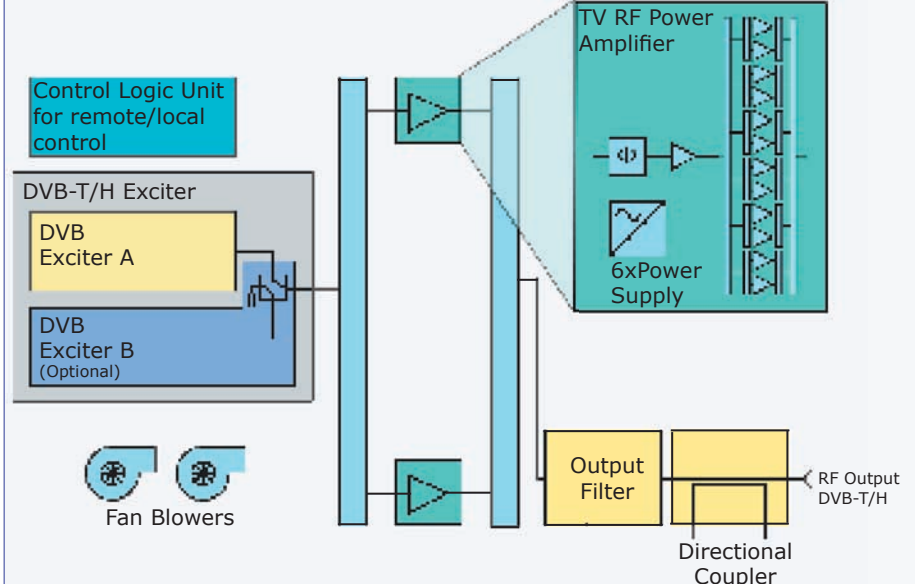
5D1K3T - Functional Block Diagram
